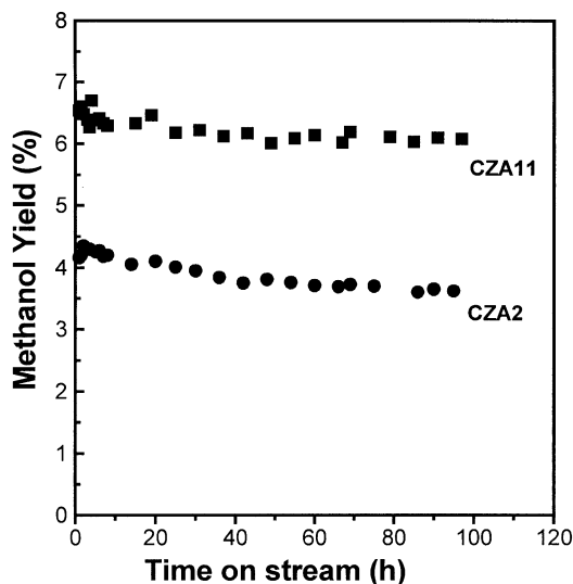
Figure 7. Methanol synthesis activity of Cu/ZnO/Al 2 O 3 catalysts prepared by various methods as a function of time on stream. Reaction conditions: T = 250\text{ }^{\circ}\text{C} , P = 2.0\text{ MPa} , F/W = 3600\text{ h}^{-1} , \text{CO}_2/\text{H}_2 = 1/3 .
