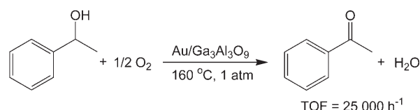
Scheme 1. Solvent-free aerobic oxidation of (±)-1-phenylethanol using an Au/Ga 3 Al 3 O 9 catalyst. Turnover frequency given for the following conditions: measuring time t = 30 min, (±)-1-phenylethanol (165.7 mmol), Au ( 4.0 \times 10^{-4} mol%).
